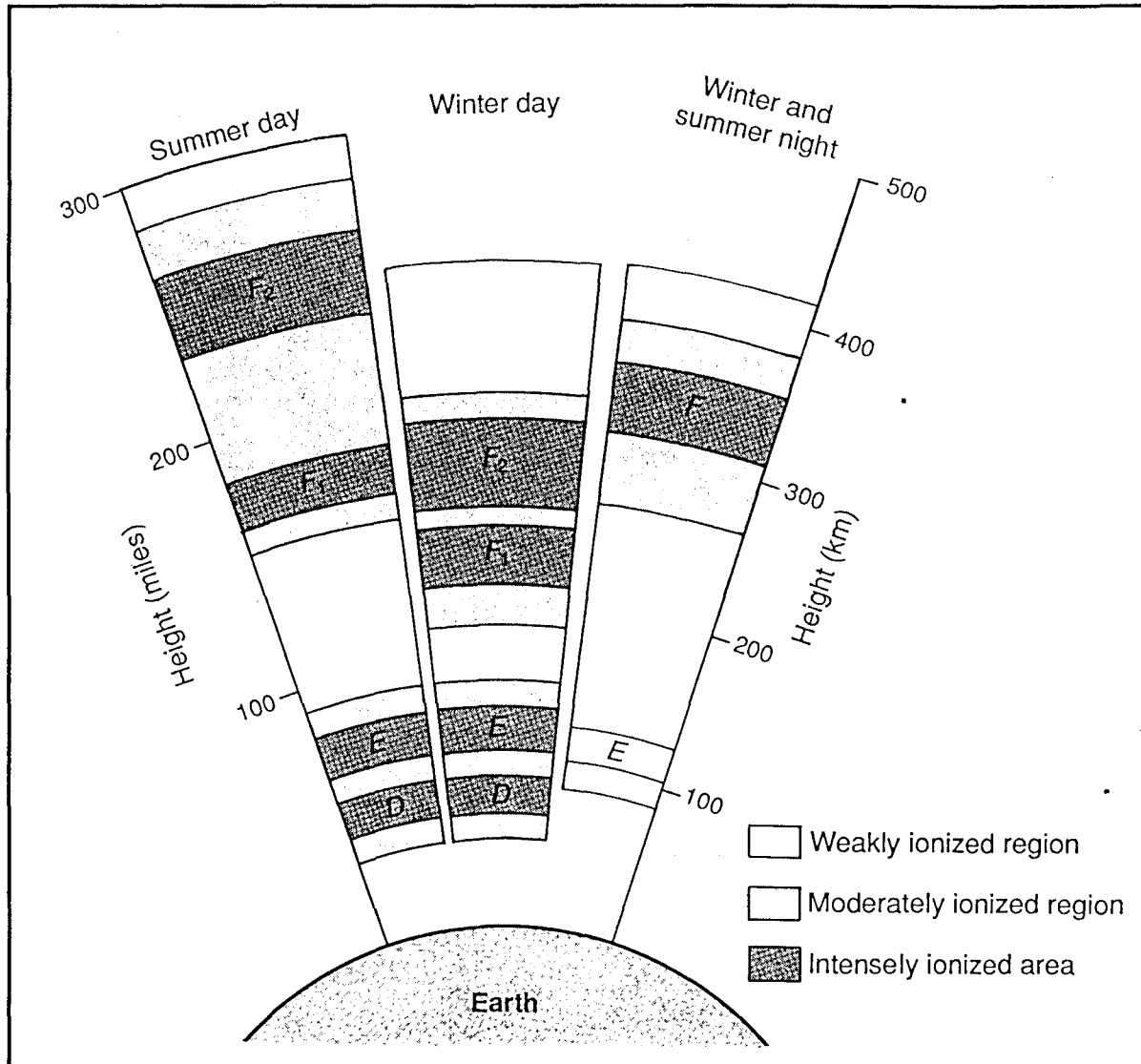
Figure 1.6. Daily and seasonal variations in the ionospheric regions (typical characteristics shown). Note that there is some residual ionization in the E layer during the nighttime hours.
