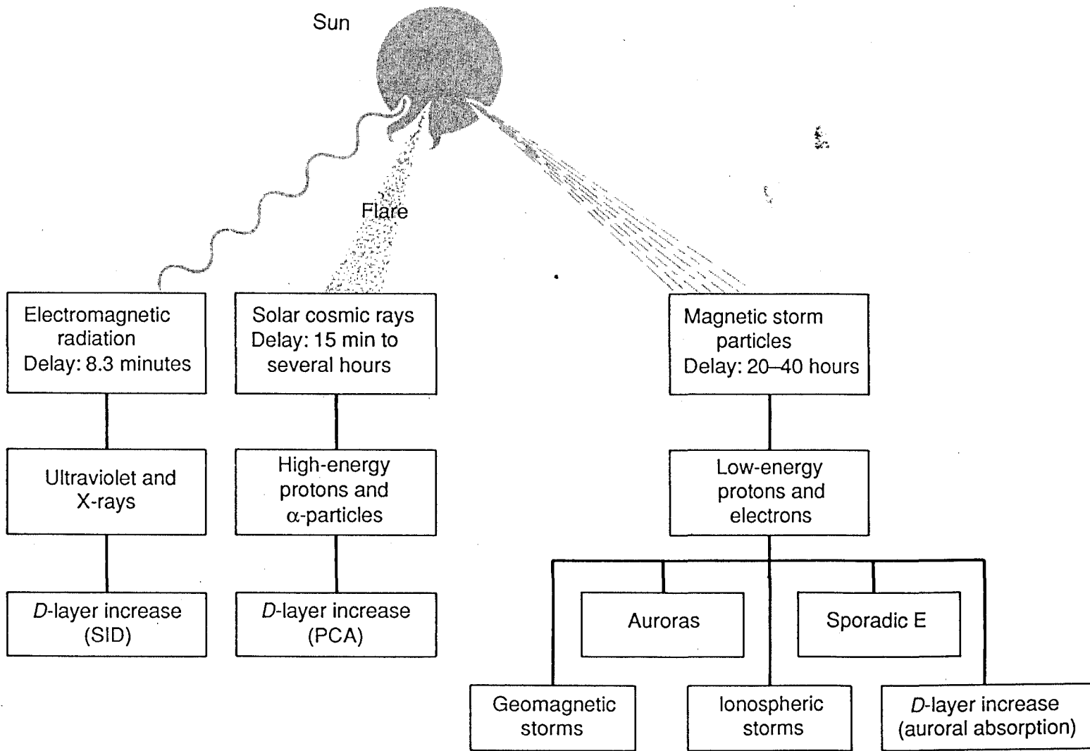
Figure 1.18. Flare emissions and ionosphere effects. (Modified after R. W. Knecht [unpublished]; see also Reference 12.)
